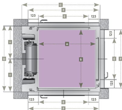
Built shaft
