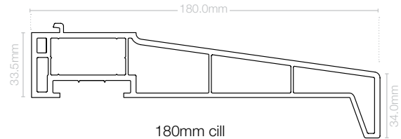
180mm cill VSW008
