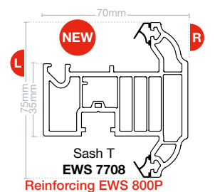
NEW Sash T EWS 7708 Reinforcing EWS 800P
