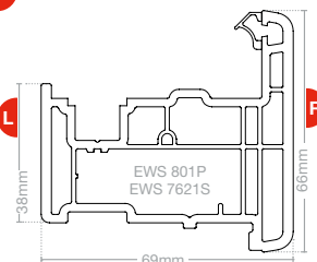
French door mullion LSF 1016
