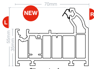
NEW Slim outer frame EWS 7720 Reinforcing EWS 800P
