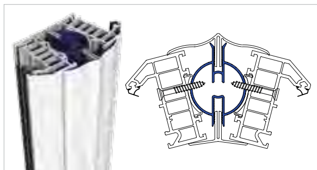
Variable bay post assembly 150-170° angles
