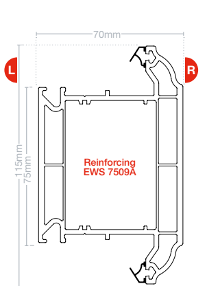
Reinforcing EWS 7509A Door mid rail EWS 7709
