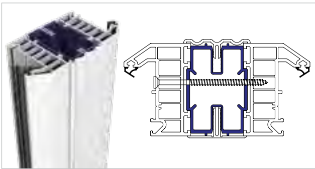
Structural butt joint assembly with sculptured trim
