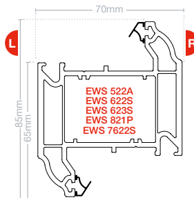
EWS 522A EWS 622S EWS 623S EWS 821P EWS 7622S Intermediate transom Z EWS 7723
