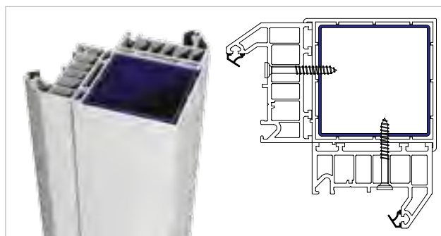
70mm square bay post assembly 90° angle
