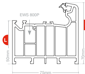
Large main frame LSF 1006
