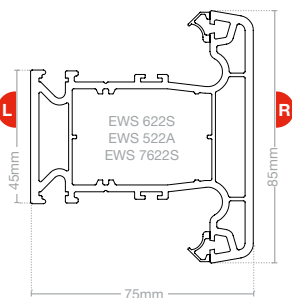
Intermediate Transom T LSF 1022
