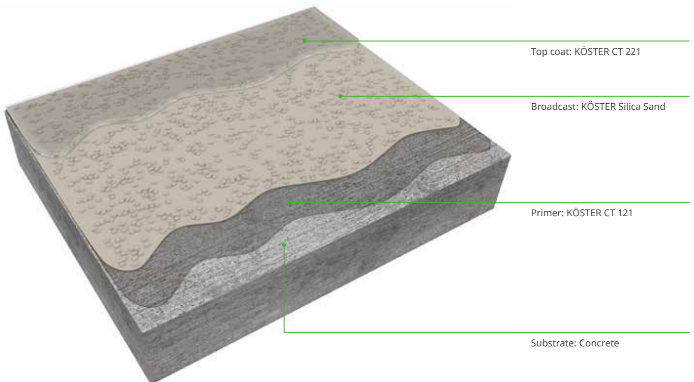
KÖSTER OS 8 System, Panama Parking of St. George Bank
