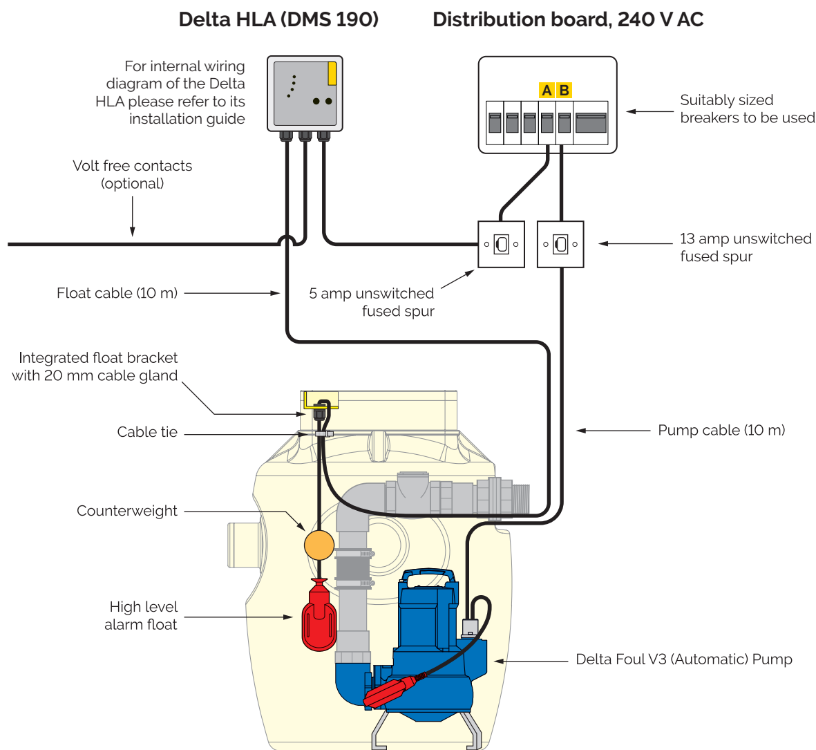
Delta Foul V3 packaged pumping station (DMS 165)
