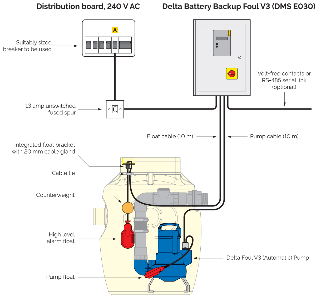
Delta Foul V3 packaged pumping station (DMS 165)
